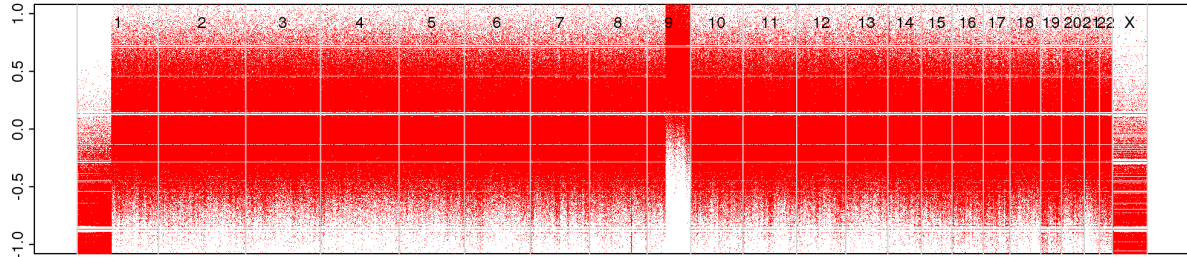
Patient 10, tumor data, BAF
